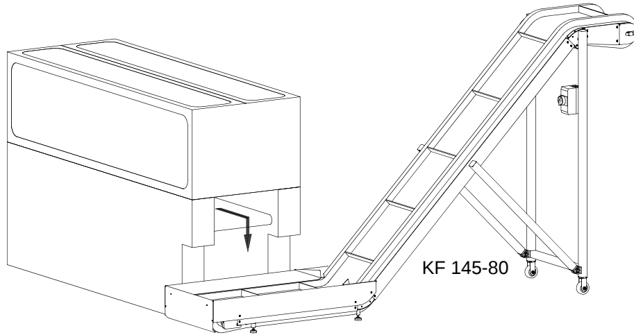
Waste conveyor with lengthened delivery chute of 800 mm
