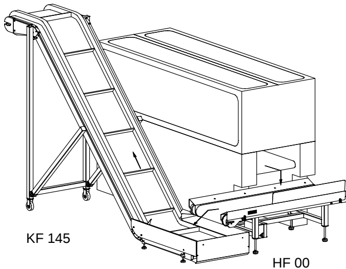
Combination for three-knife trimmer with internal conveyor
